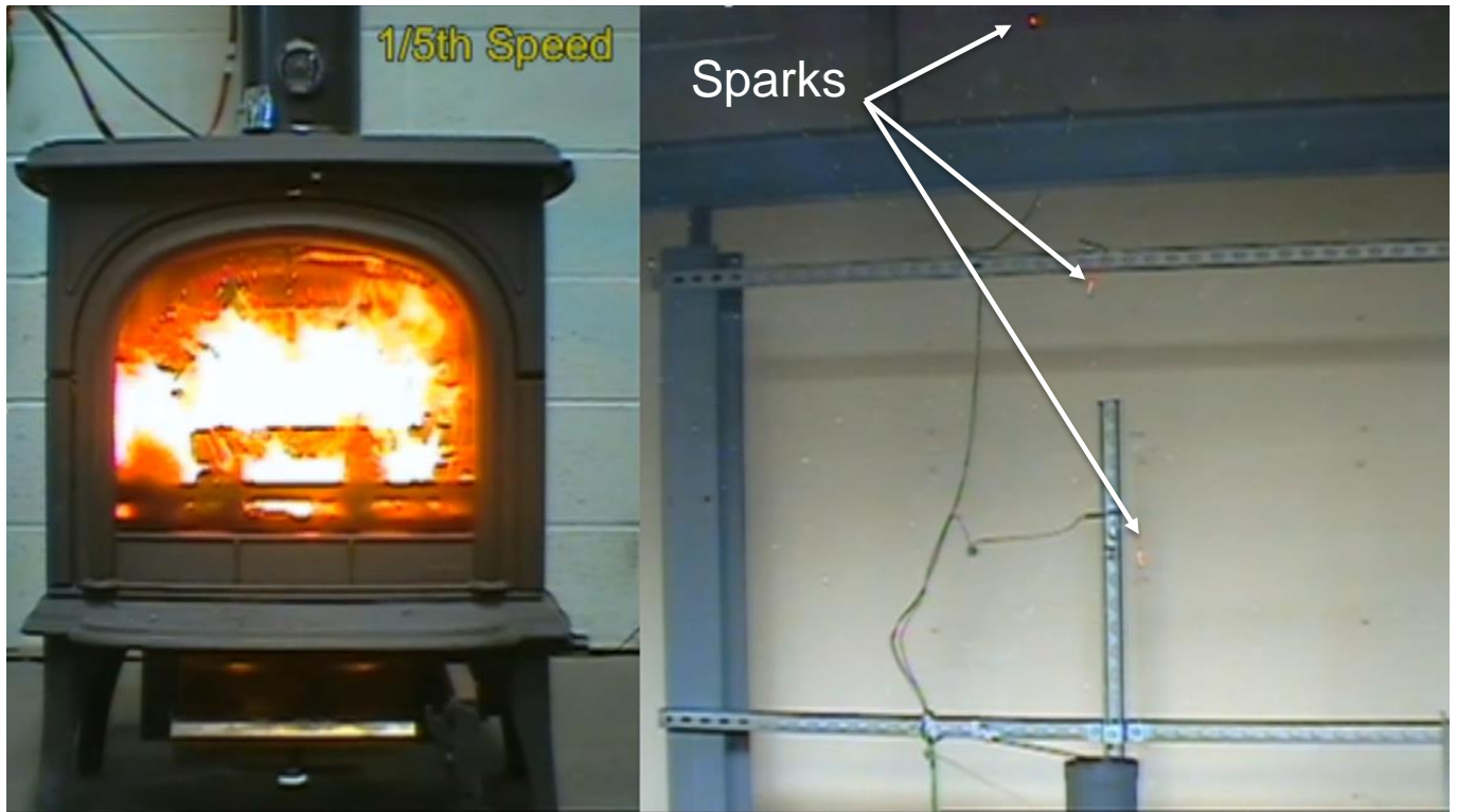
Figure 29 - Spark emission during aggressive ventilation of the stove with the ash-pan door open
