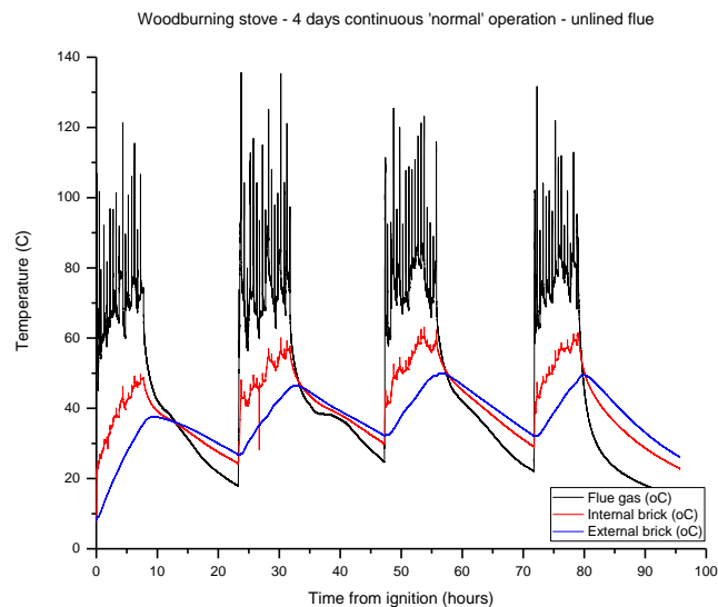
Figure 39 - Long Duration conduction investigation for an unlined chimney
