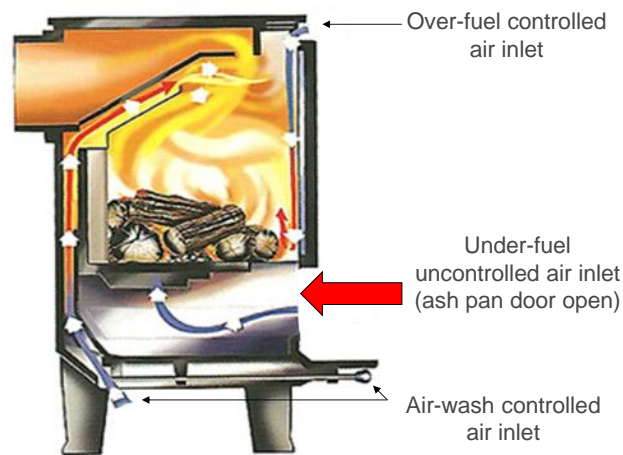
Figure 4 - Ventilation of a multi-fuel stove using the ash-pan door
